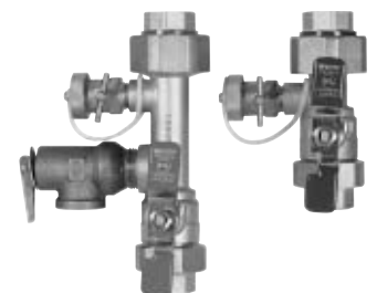
Double Union Service Valve Set Union connections to water heater and water supply line
